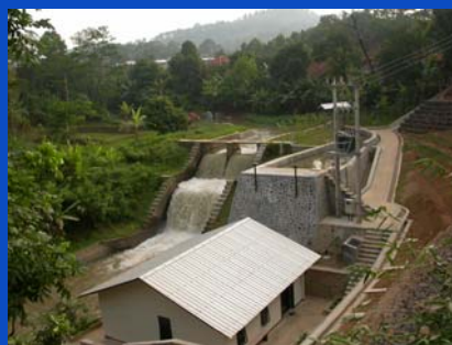
Melong, Subang, Jabar X-flow T-14 D500, ELC-100 kW-Grid PLN 2005
